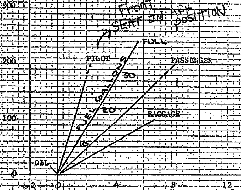
FIGURE 1-LOADING GRAPH
